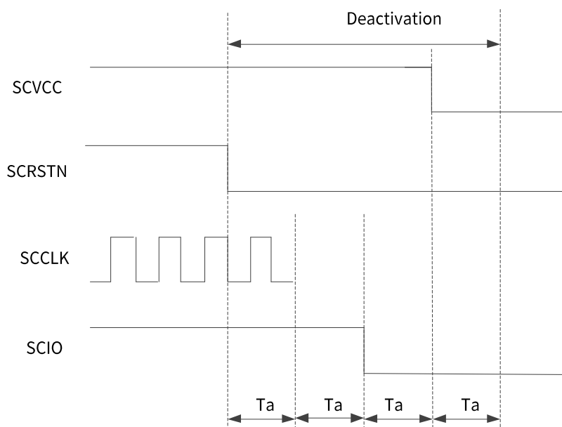
图36. Deactivation Sequence
