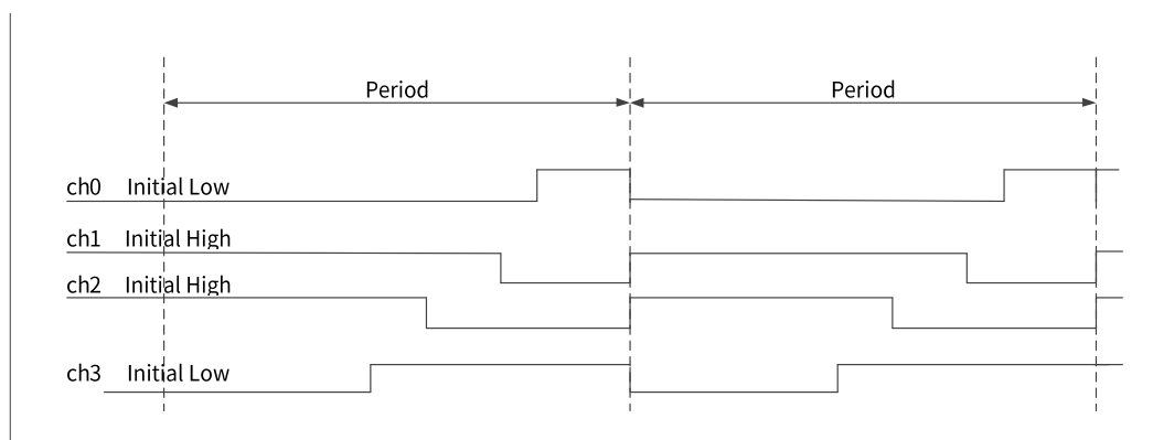
图18. Edge-aligned PWM
