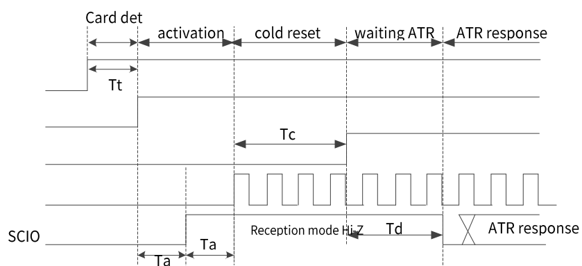
图35. Activation, Cold Reset and ATR
