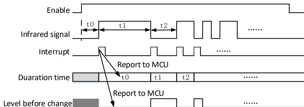
图40. IR Receiver
